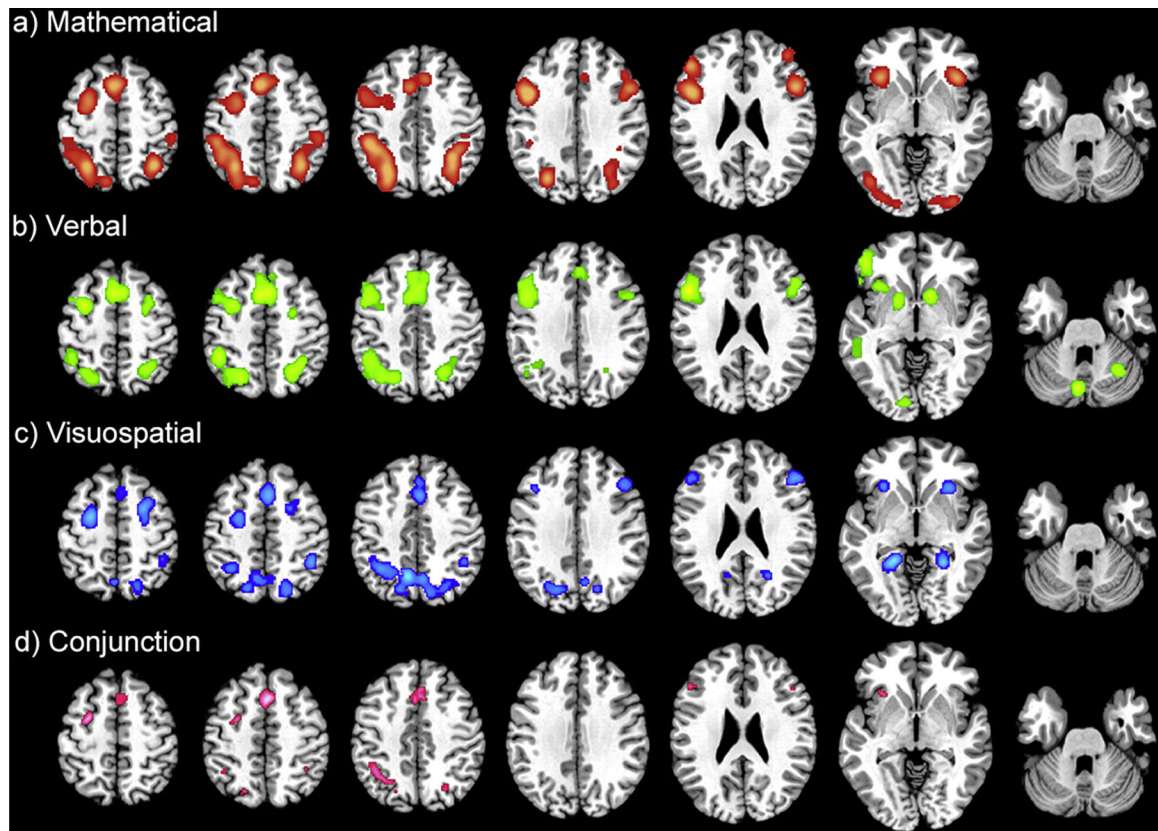
Fig. 2. Representational Domain-specific and Conjunction Problem Solving Meta-Analyses. Problem solving experiments were categorized into three representational variants. Within-domain meta-analytic maps are shown for (a) mathematical problem solving (red) = 99 experiments, (b) verbal problem solving (green) = 93 experiments, and (c) visuospatial problem solving (blue) = 88 experiments. A common set of brain regions, present across this heterogeneous set of 280 problem solving contrasts, is depicted in (d), which shows the minimum statistical conjunction between all three within-domain maps (pink) (For interpretation of the references to colour in this figure legend, the reader is referred to the web version of this article.).
