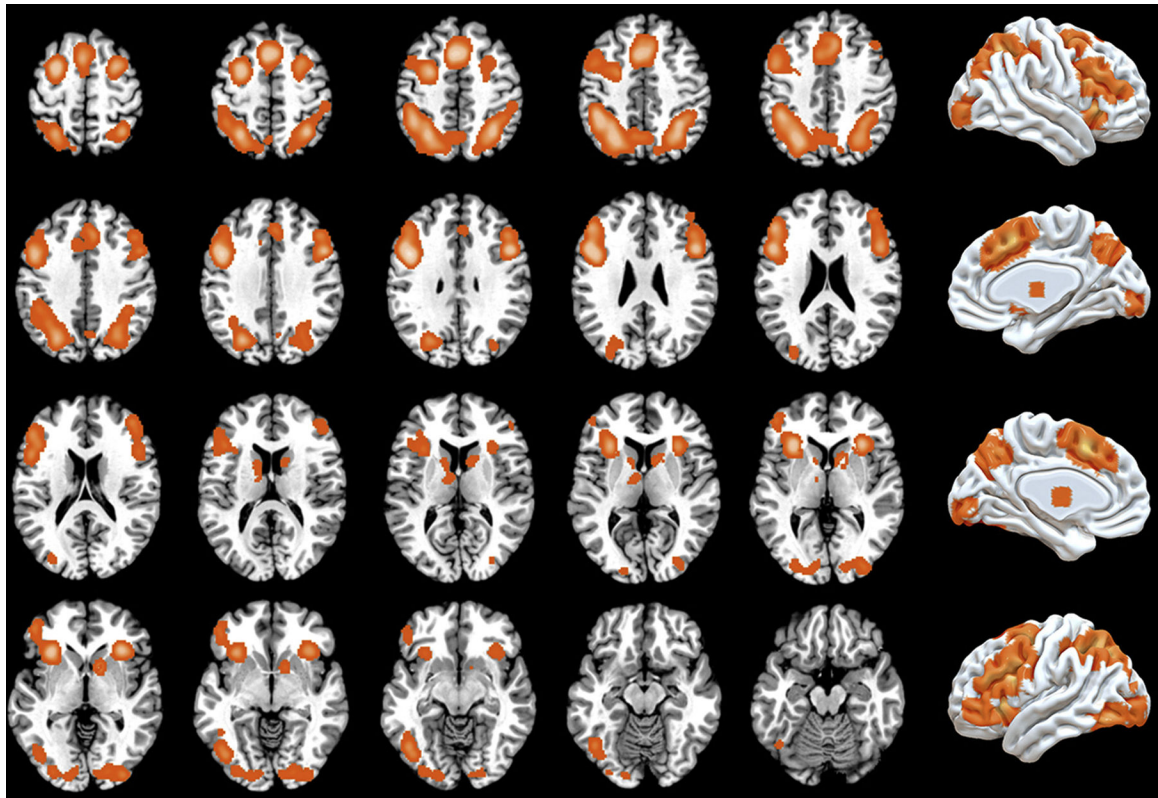
Fig. 1. Global Problem Solving Meta-Analysis. The global problem solving meta-analysis identified convergence across 131 papers reporting coordinate results from a diverse range of problem solving experiments. Multiple problem solving modalities were represented in this set, with 280 experimental contrasts across 1919 subjects. The broad engagement across whole-brain systems depicted by this map represents the overall neural underpinnings of problem solving.
