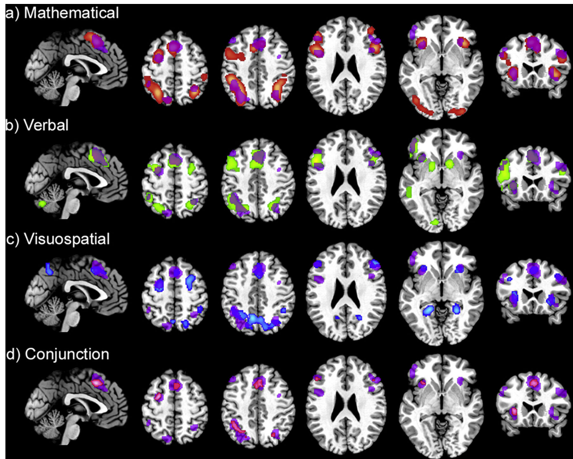
Fig. 4. Problem Demand Meta-Analyses and Domain-Specific Overlays. High vs. low demand problem solving meta-analysis (= 41 experiments), as compared across problem solving by representational domains. Meta-analysis of problem solving tasks contrasting high vs. low demand (transparent purple) are overlaid with the three representational domain meta-analysis and the conjunction meta-analysis: (a) mathematical domain (red), (b) verbal domain (green), (c) visuospatial domain (blue), and (d) conjunction across domains (pink).
